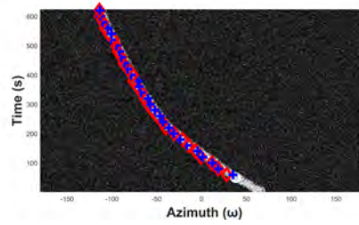
(c) Conventional: SNR = -8 dB
