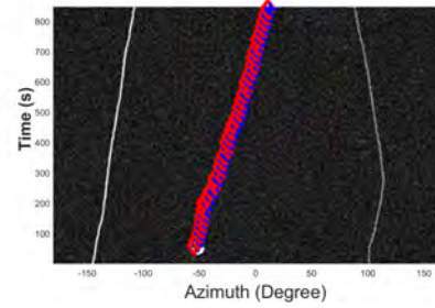
(f) Proposed: SNR = -21 dB
