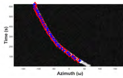
(a) Conventional: SNR = 3 dB
