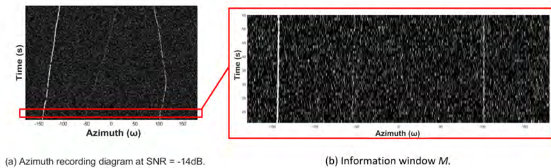
Figure 15. Information window extraction.
