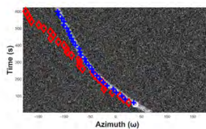
(i) Conventional: vSNR = -21 dB
