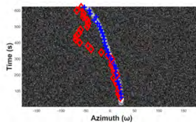
(i) Conventional: SNR = -21 dB
