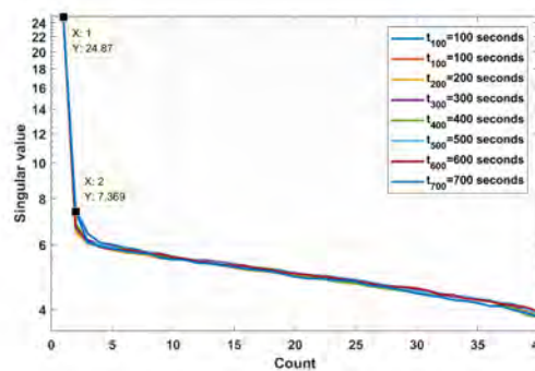
Figure 16. Singular value vectors.
