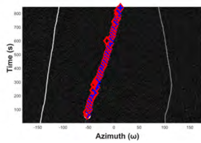
(c) Conventional: SNR = -14 dB
